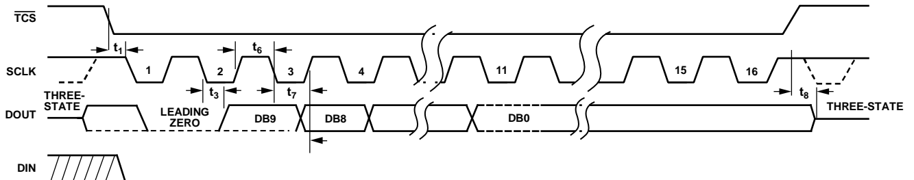
Figure 4. Temperature Serial Interface Timing Diagram
